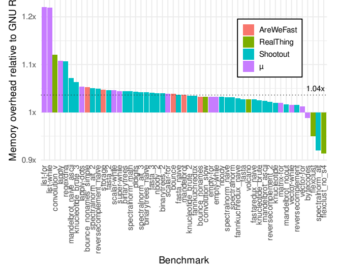
Figure 6. Memory overhead compared to GNU R. The dotted line indicates the geometric mean. Only benchmarks with differences greater than 1% are shown.
