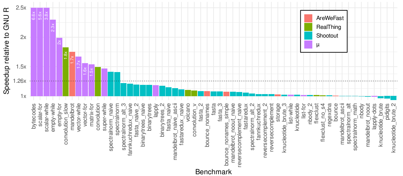
Figure 4. The speedup over GNU R. The dotted line indicates the geometric mean.
