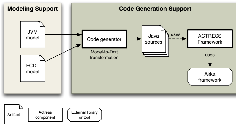
Figure 5.4: Overview of the ACTRESS code generation support
