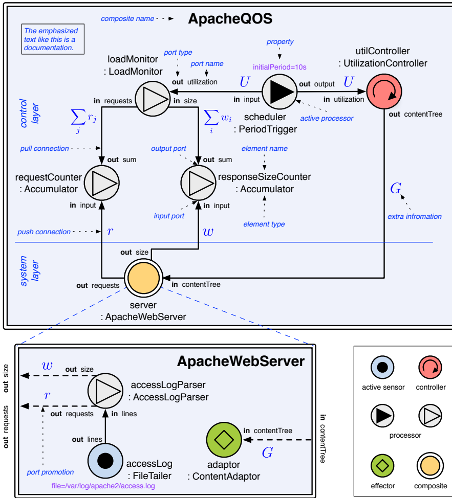
Figure 3.3: FCDL schema of the running example
